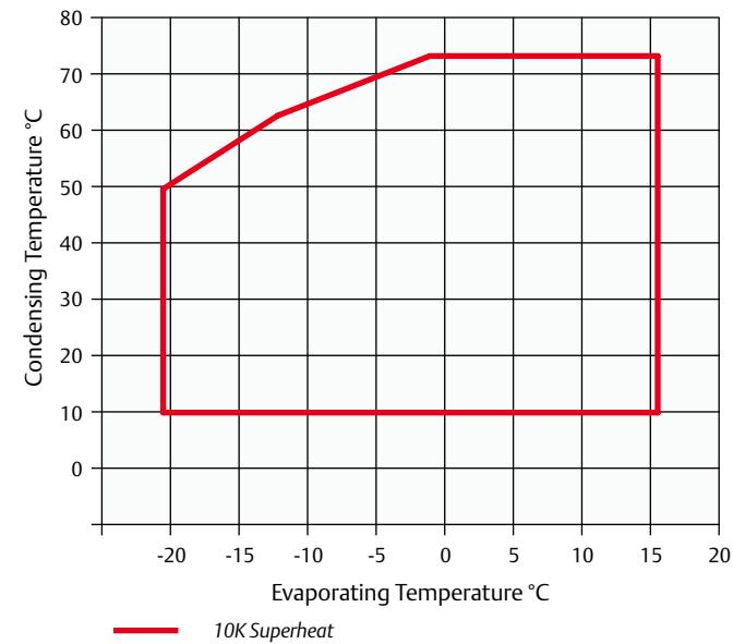
Operating Envelope R134a - For ZBD Digital Models
