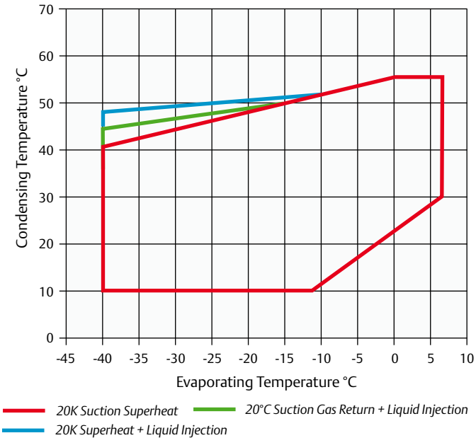
Operating Envelope R448A/R449A - For ZFD Digital Models
