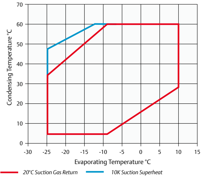
Operating Envelope R448A/R449A - For ZBD Digital Models
