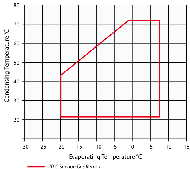
Operating Envelope R134a
