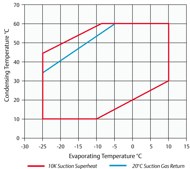
Operating Envelope R407F
