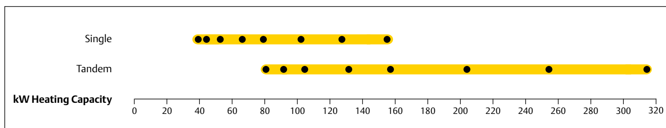
ZH*KCE Scroll Compressor For Heat Recovery
