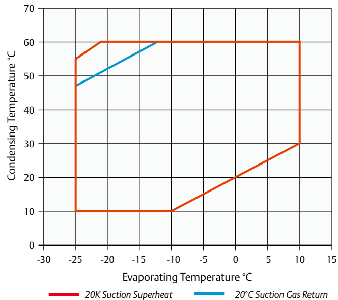
Operating Envelope R404A
